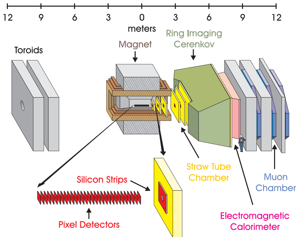
Fig. 1. Schematic view of the BTeV Spectrometer
